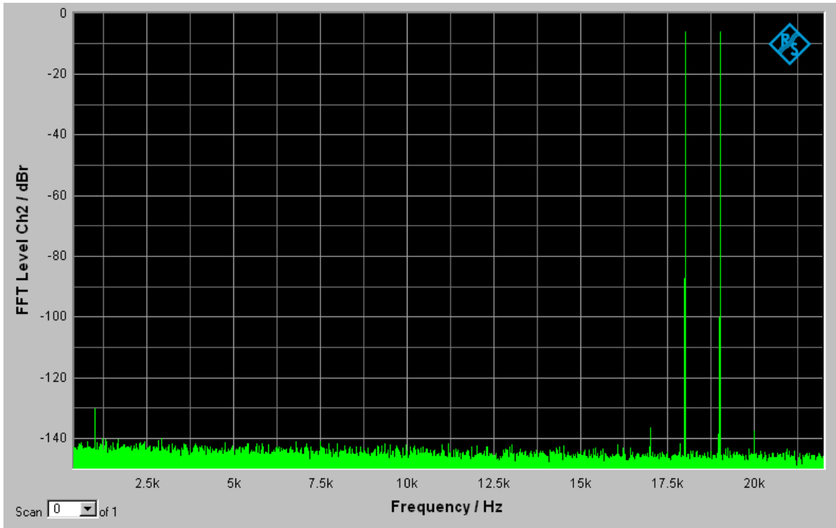
Intermodulation distortion (IMD): 18+19kHz
