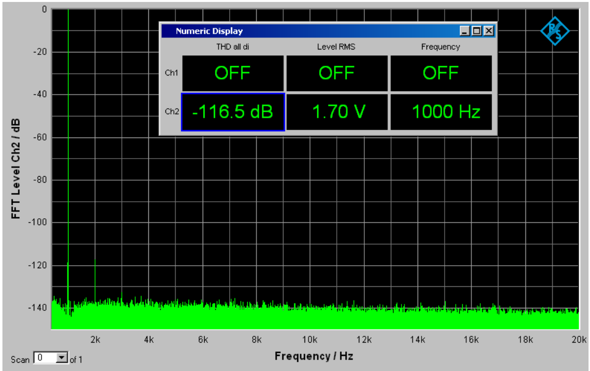
Total harmonic distortion (THD): 1kHz tone, 0dBFS, 32 ohm load (90 mW)
