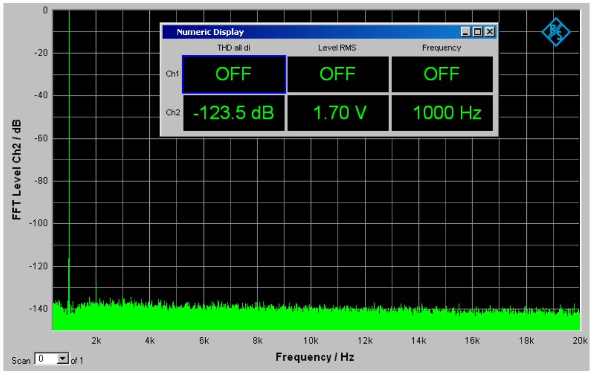
Total harmonic distortion (THD): 1kHz tone, 0dBFS, 600 ohm load (5 mW)
