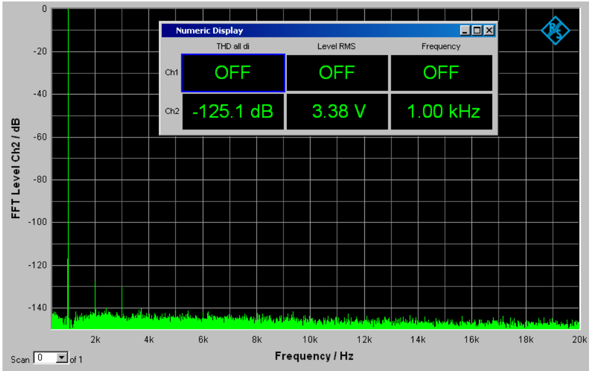
Total harmonic distortion (THD): 1kHz tone, 0dBFS
