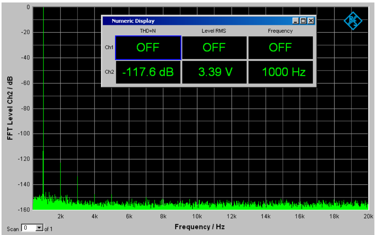
Total harmonic distortion + noise (THD+N): 1kHz tone, 0dBFS, 20kHz BW
