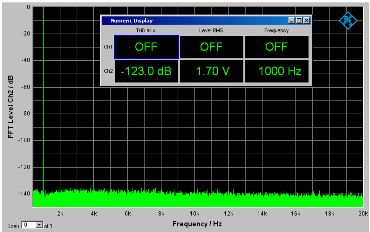
Total harmonic distortion (THD): 1kHz tone, 0dBFS, 300 ohm load (10 mW)
